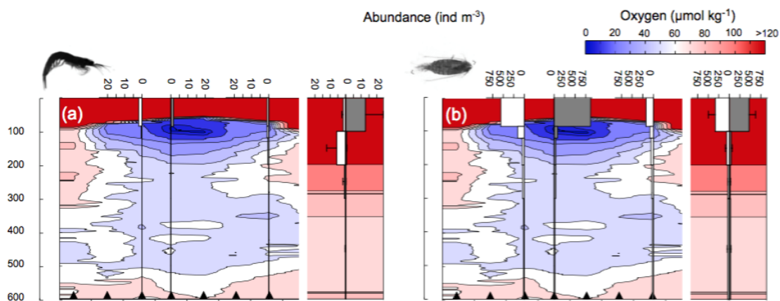
Figure 14b: Low oxygen eddy off West Africa: Oxygen contours ( \mu\text{mol O}_2 \text{ kg}^{-1} ) across a low oxygen eddy (from NE to SW) with superimposed bar plots of multinet-based abundance (individuals \text{m}^{-3} ) of euphausiids (a), and calanoid copepods (b). A very sharp oxycline is found at 60m depth (from saturation ( >250 \mu\text{mol kg}^{-1} ) to 5 \mu\text{mol kg}^{-1} over a distance of 10 m. White and grey bars indicate daylight and nighttime hauls, respectively. Triangles denote CTD stations used for the \text{O}_2 section. (see Hauss et al. 2016; data sets: https://doi.pangaea.de/10.1594/PANGAEA.858323 )
